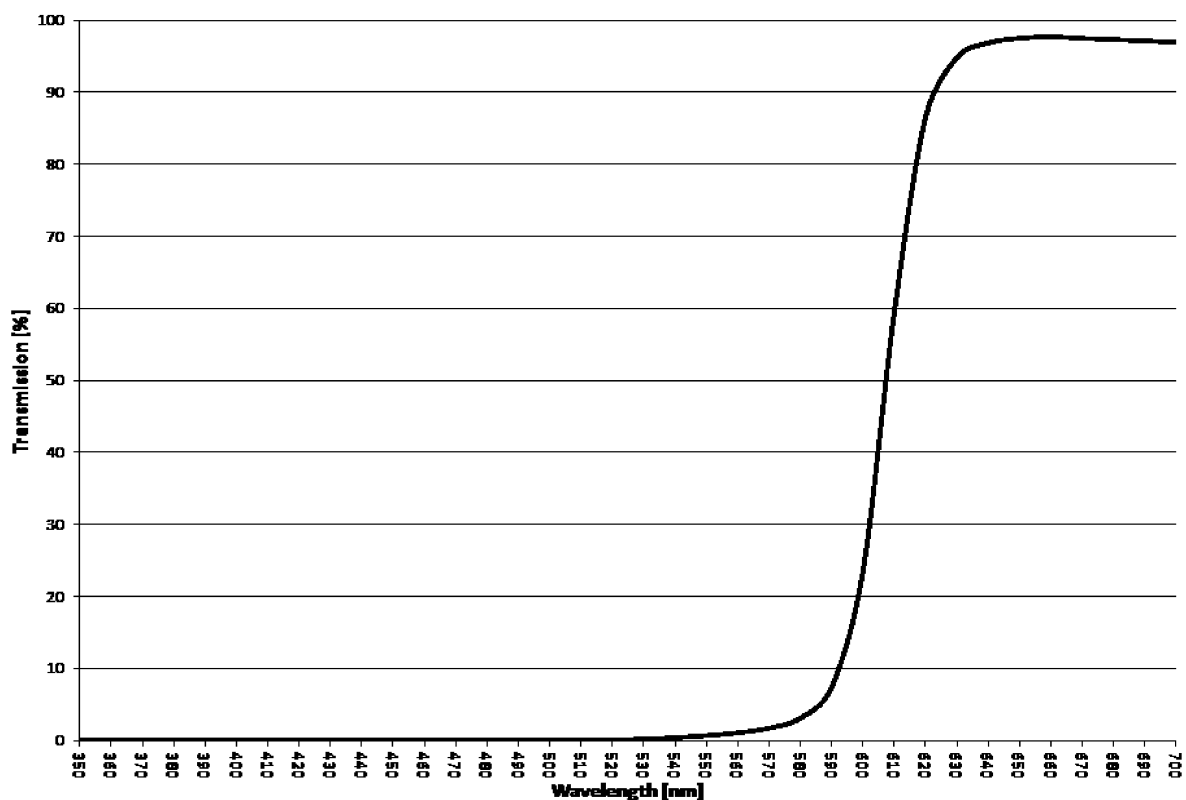
Spectral Transmittance
